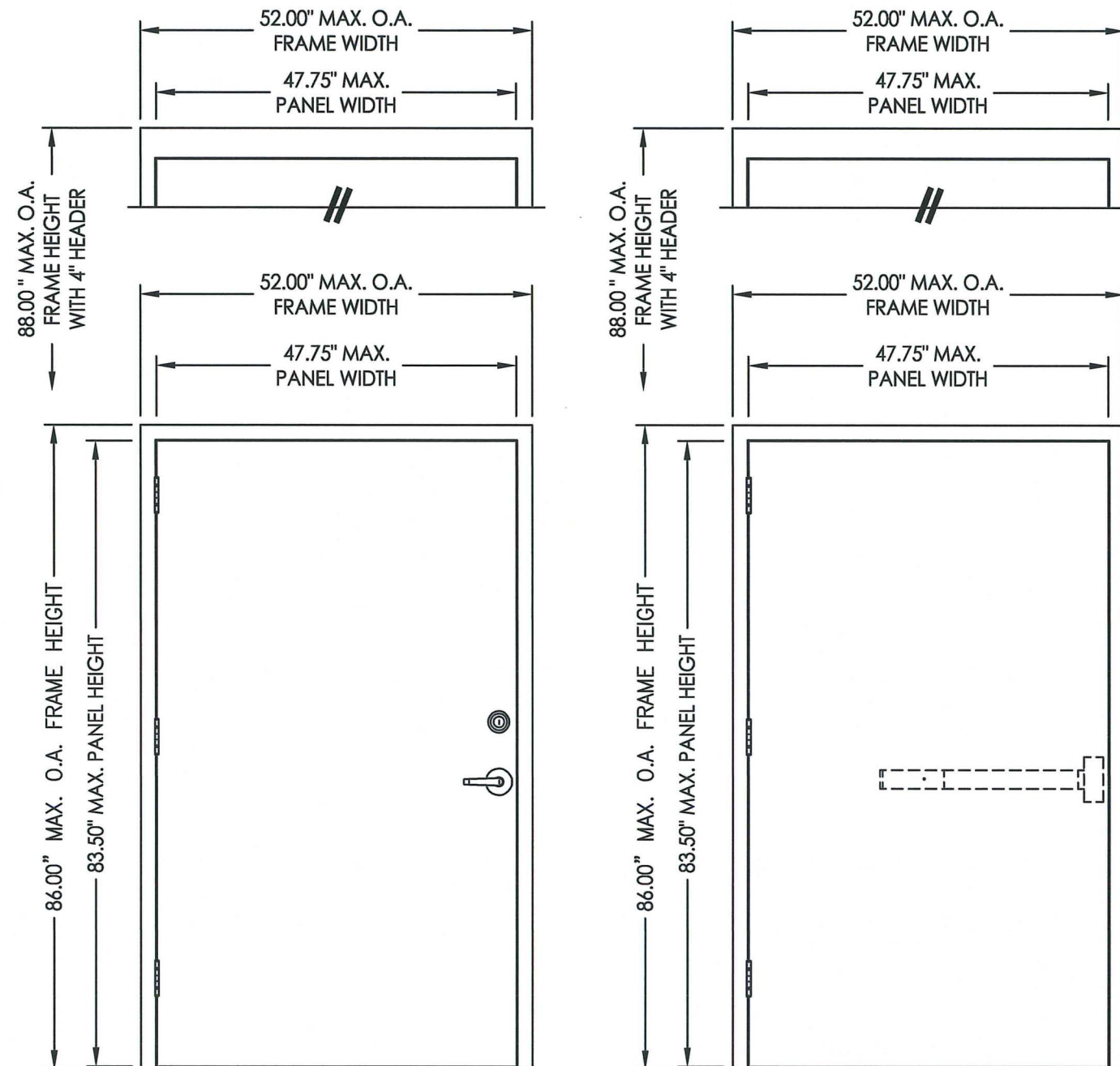
"N" DOOR
